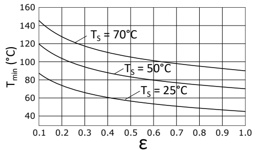
Graph showing the minimum measurable object temperature ( T_{min} ), determined by surface emissivity ( \epsilon ) and sensor temperature ( T_s ).
